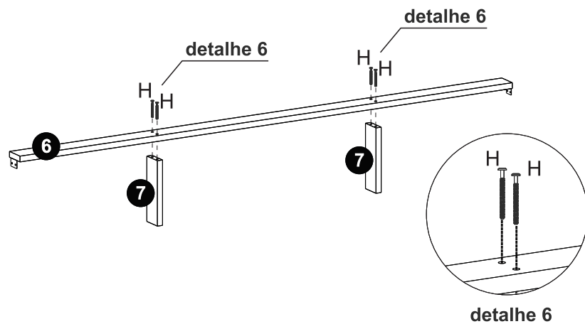
H- Parafuso 7x60 (4x)
