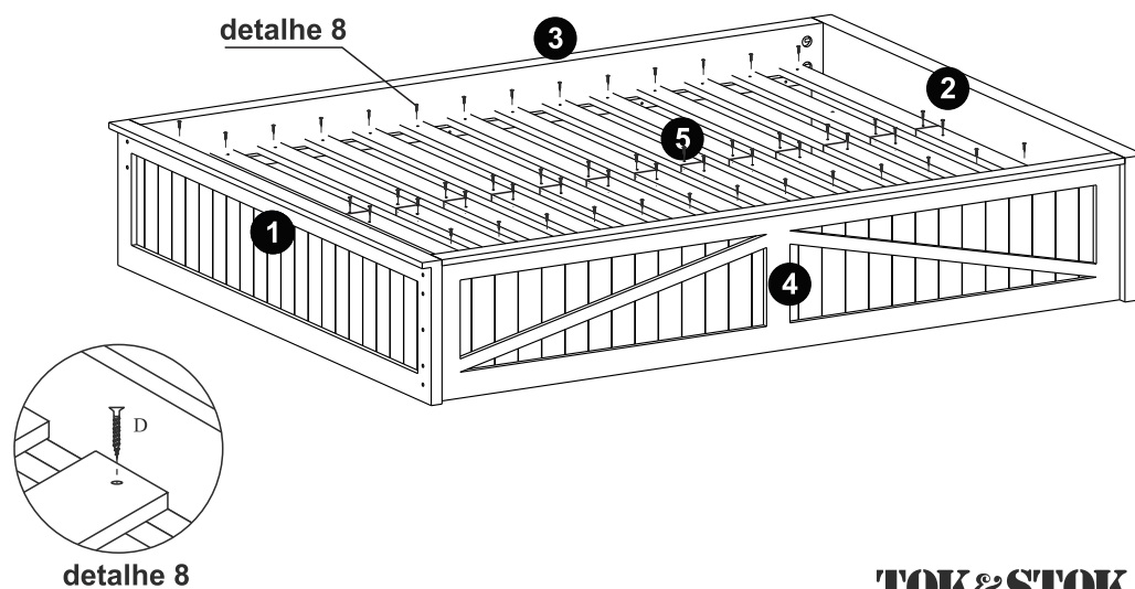
D- Parafuso ch 3,5x30 (56x)
