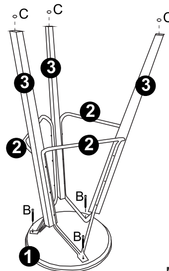
B - Parafuso Ø3,5x16 (3x)
