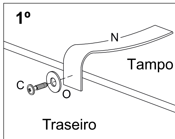
C - Parafuso Ø3,0x16mm (1x)
